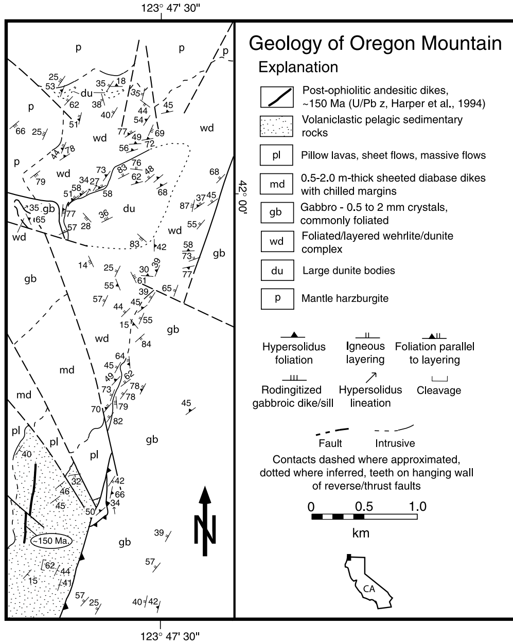
Fig. 6. Geologic map of the lower crustal section exposed at Oregon Mountain displaying structural and lithologic elements within the wehrlite–dunite and gabbro sequences. Only the largest dunite bodies are shown on the map; generally these bodies consist of mixed dunite and wehrlite at the 1–10 m scale.
