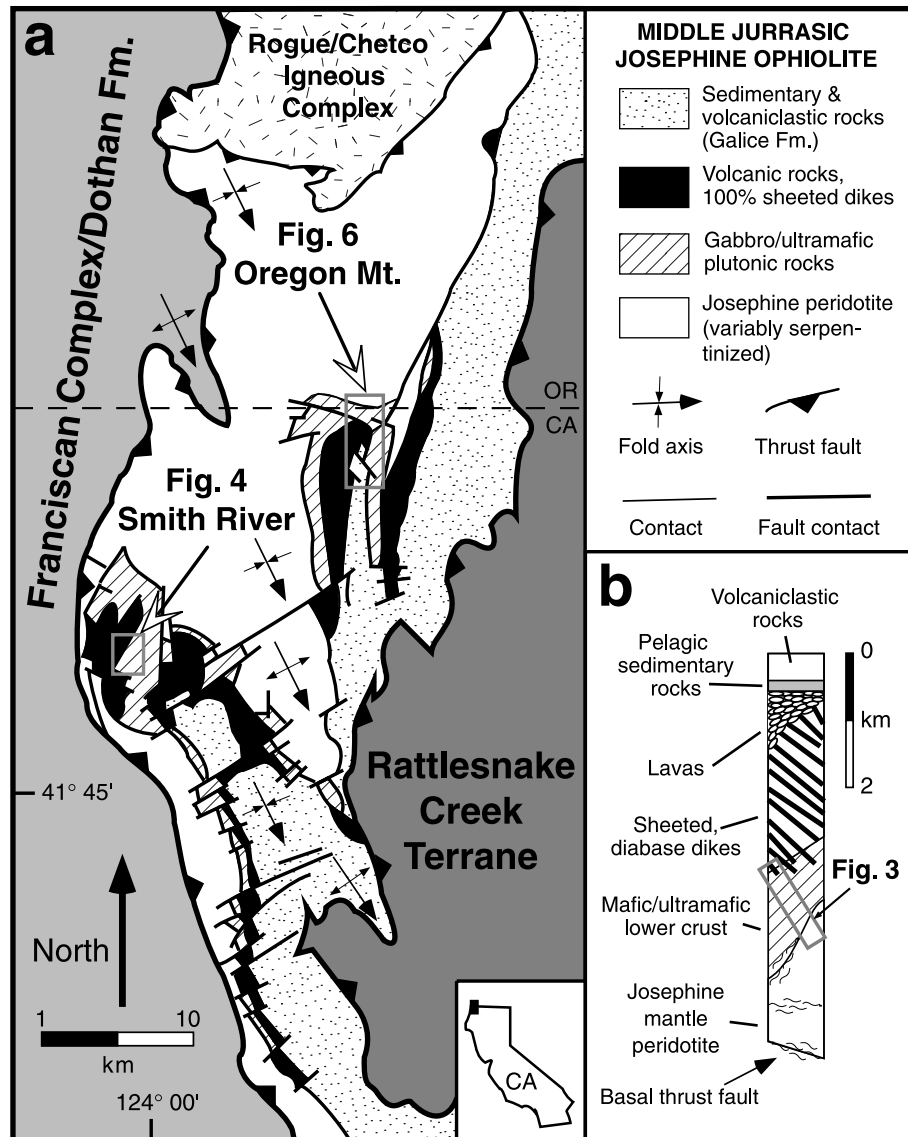
Fig. 2. (a) Simplified geologic map of the Josephine ophiolite (modified from Alexander and Harper, 1992); (b) generalized crustal column for the Josephine ophiolite; note that pillow lavas and flows have steeper dips down section, implying eruption during growth faulting.
